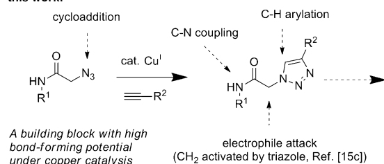
Scheme 1. Merging of copper-mediated cross-coupling and cycloaddition reactions by a “click-and-activate” protocol.
